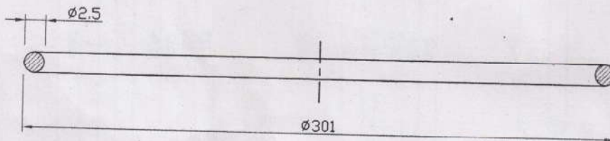
ITEM 2 'O' RING - CYLINDER TUBE Qty. Reqd : 2Nos.
